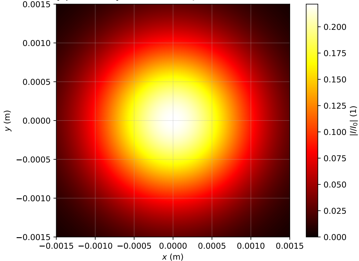
Intensity profile I(x, y, z = 3.981m)/I_0 , Pin=0.1Pcr, artificial time
